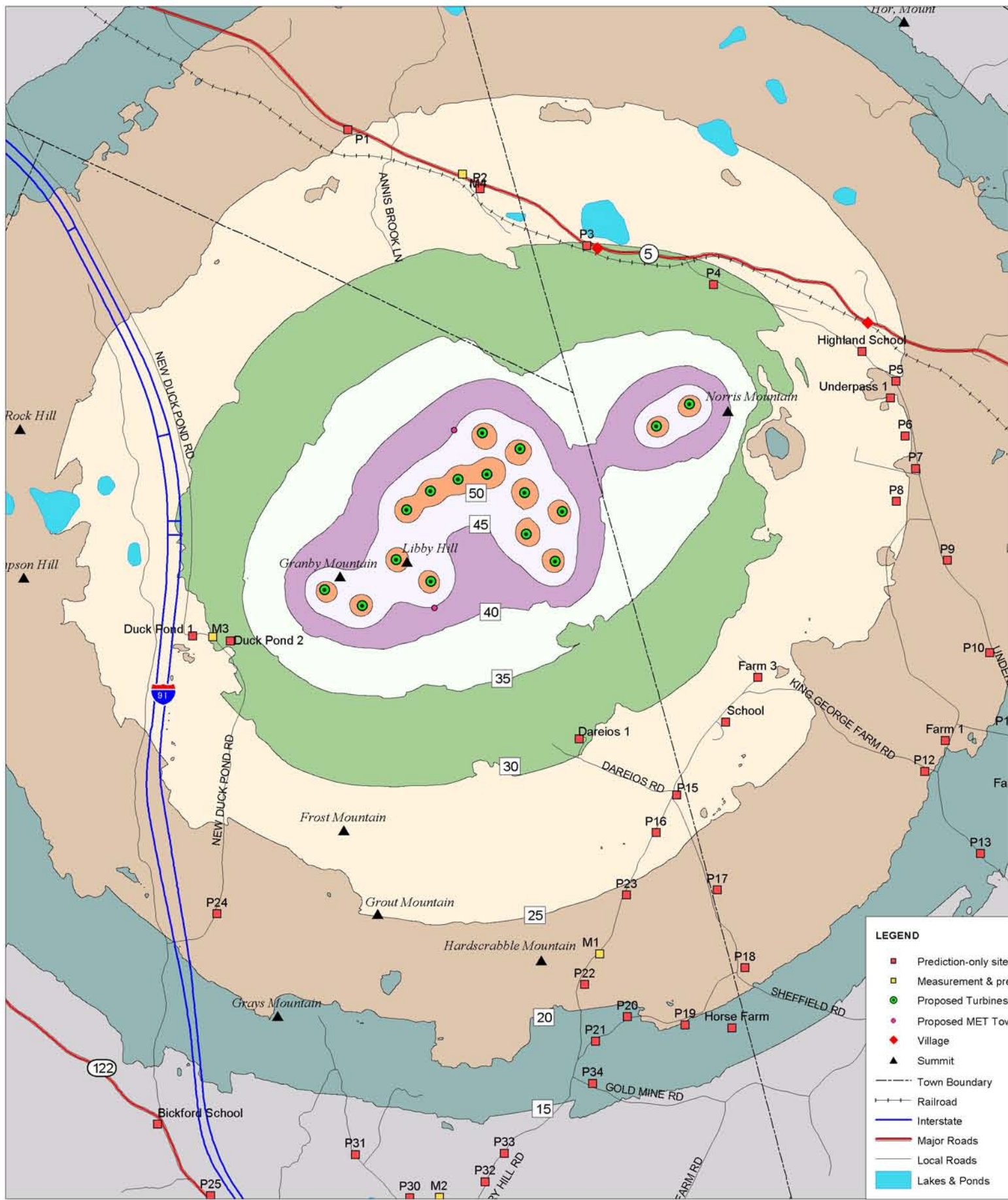
NOISE STUDY WITHOUT FOREST SHEFFIELD WIND FARM Revised Turbine Layout
