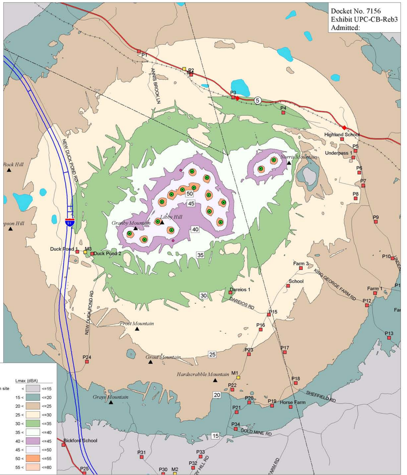
NOISE STUDY WITH FOREST SHEFFIELD WIND FARM Revised Turbine Layout
